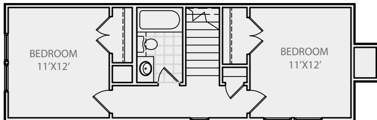
SECOND FLOOR PLAN SCALE: 3/32"=1'-0"
