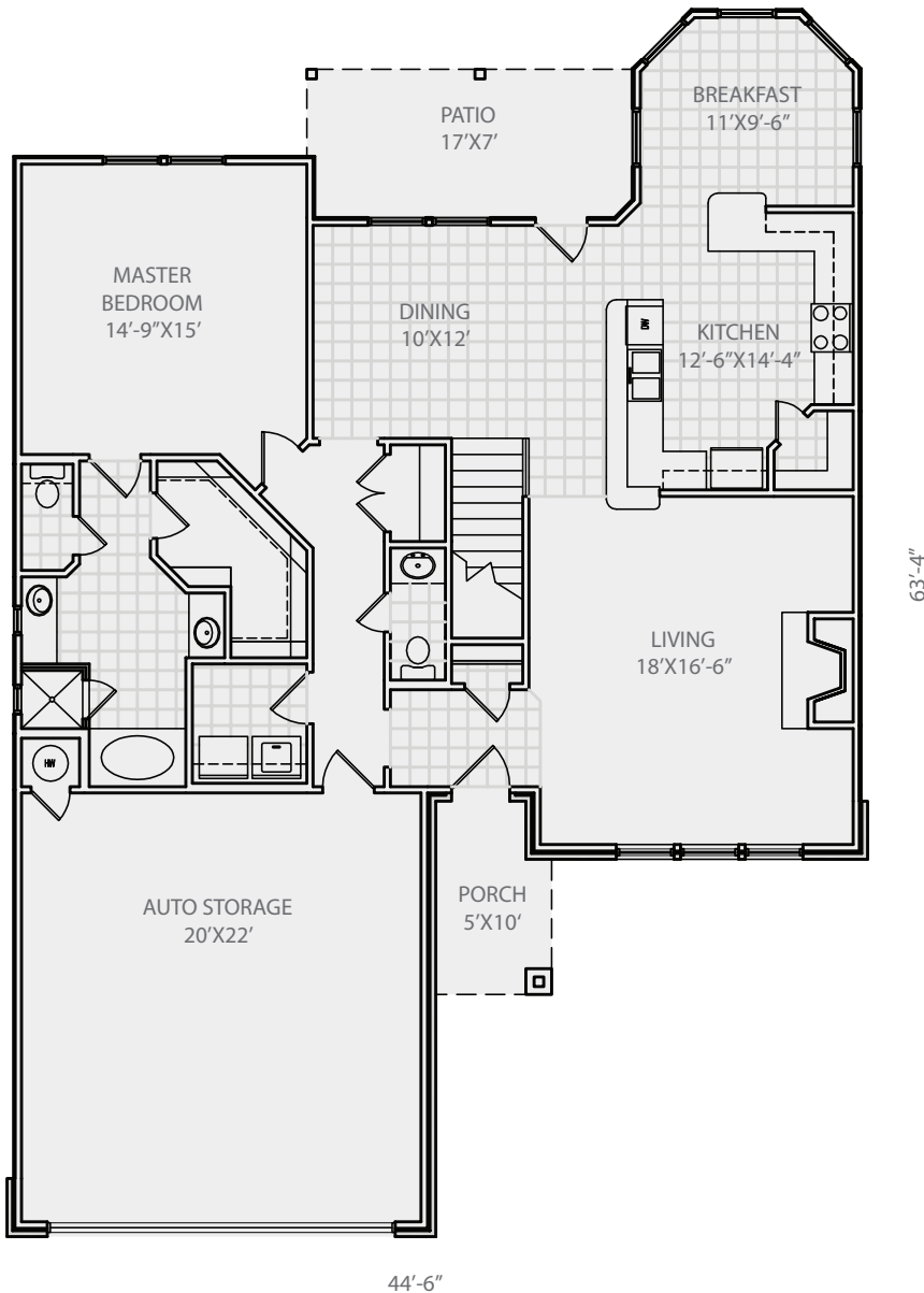
FIRST FLOOR PLAN SCALE: 3/32"=1'-0"
